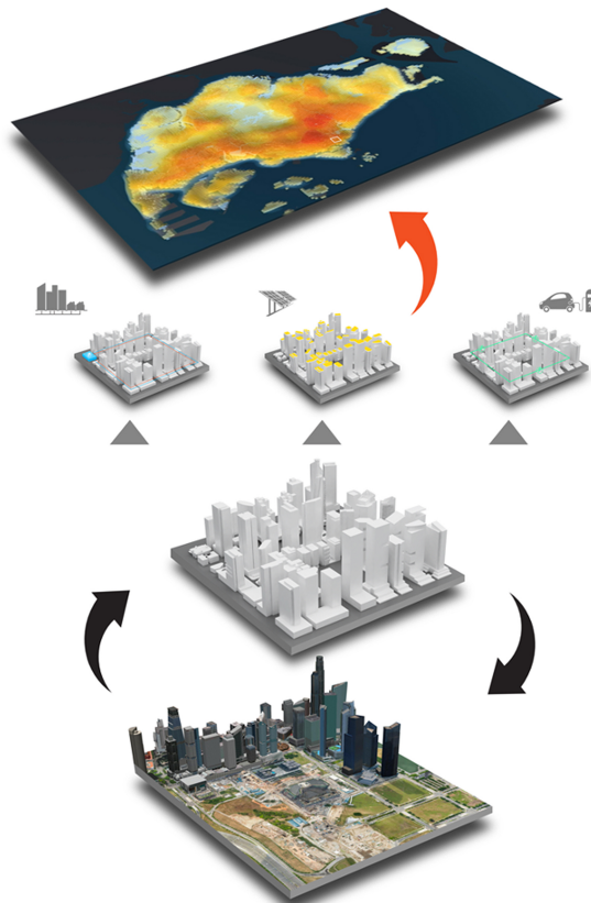
Digital Urban Climate Twin model, Cooling Singapore, 2020
